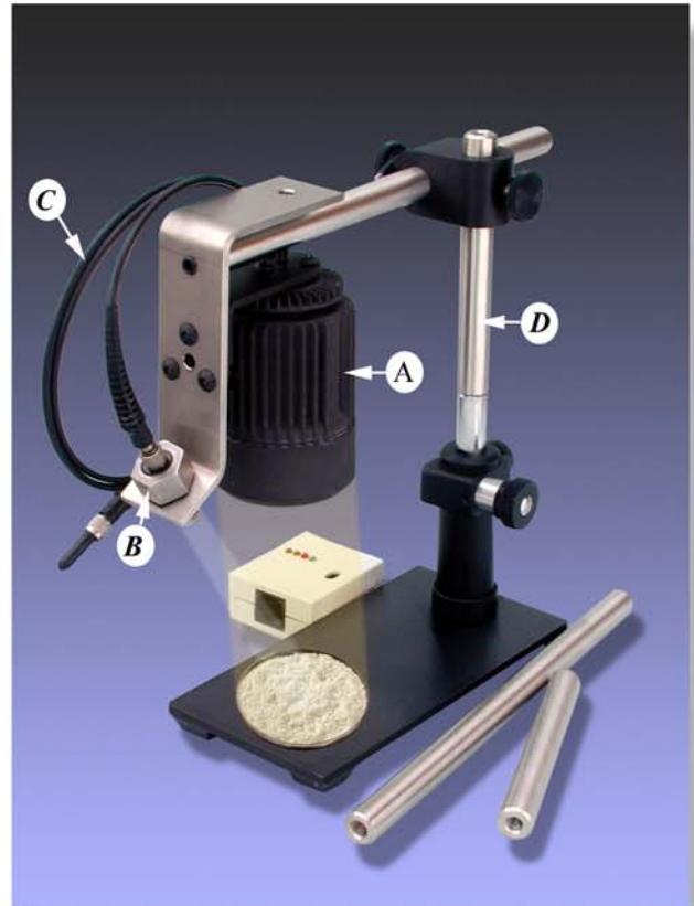
Light Fixture (*D) shown with Lamp (A), Lens (B) and Optical fiber (C).
